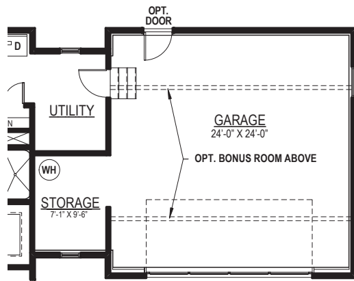
FIRST FLOOR OPT. SIDE TWO-CAR GARAGE W/ STORAGE & UTILITY ADDITION
