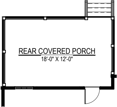
OPT. REAR COVERED PORCH
