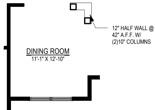
OPT. DINING ROOM W/ HALF WALLS & COLUMNS IN LIEU OF BEDROOM #2
