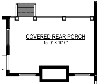
OPT. COVERED REAR PORCH W/ OPT. DBL SIDED FIREPLACE IN LIEU OF DECK
