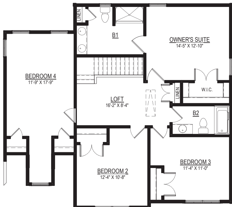
SECOND FLOOR PLAN OPT. BEDROOM #4
